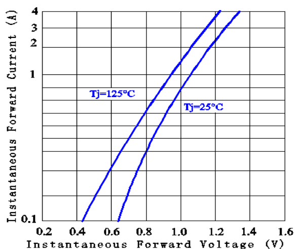
FIG3: Forward Voltage
